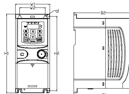
Wall mounting
